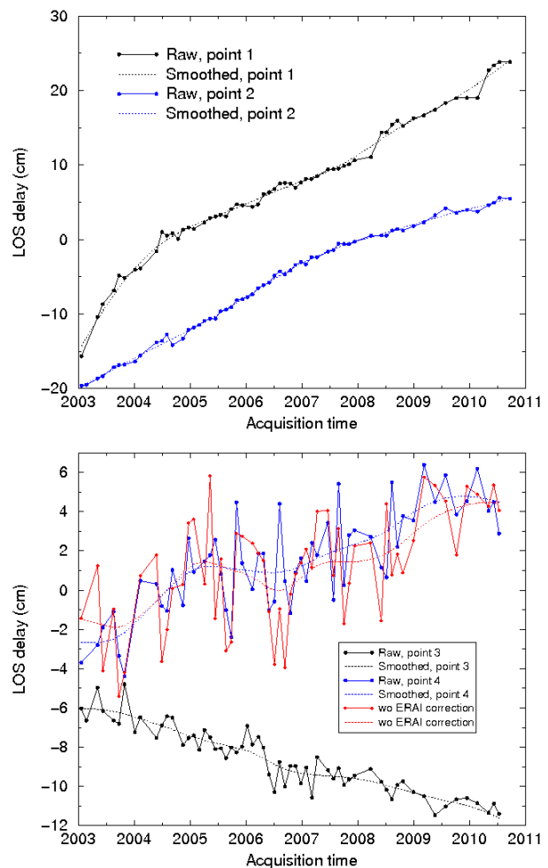
Figure 13. Displacement history of four pixels marked x on velocity map in Fig 12 relative to neighbouring pixels labeled with r. For pixel 4 the LOS delay evolution is shown with and without stratified atmospheric correction using ERAI model.
